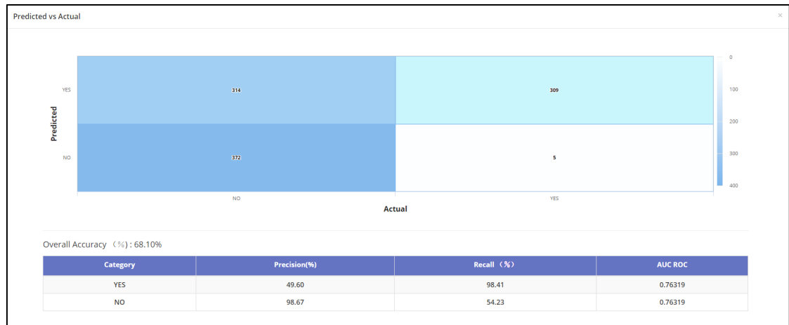
Figure 38 - Predicted vs Actual - Binary, both value prediction - Categorical
