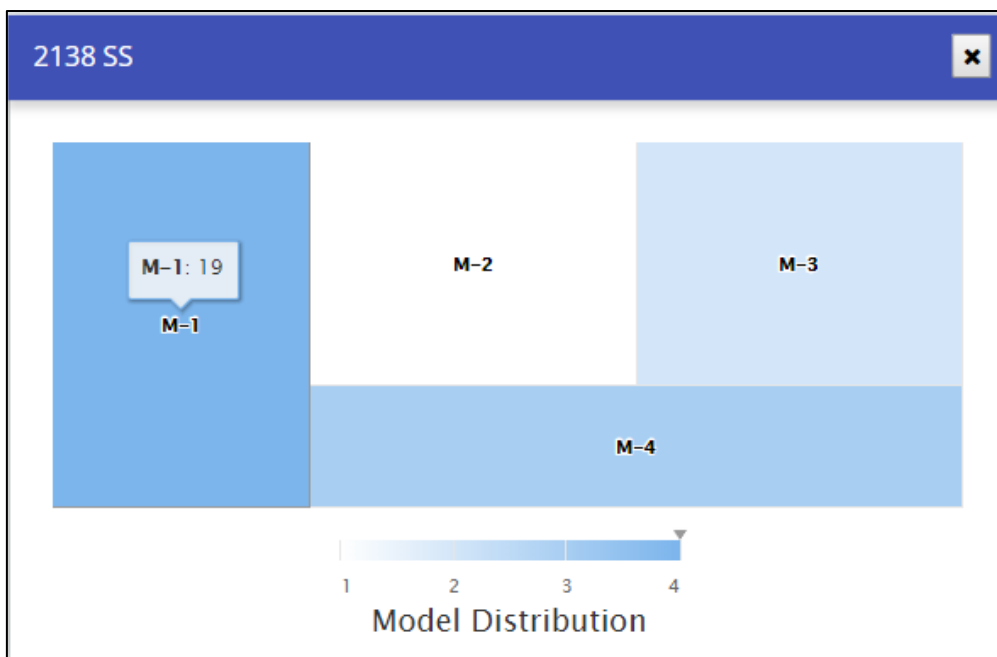
Figure 17 - MultiModel Forecast
